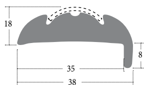
JPW9824B With Lip
