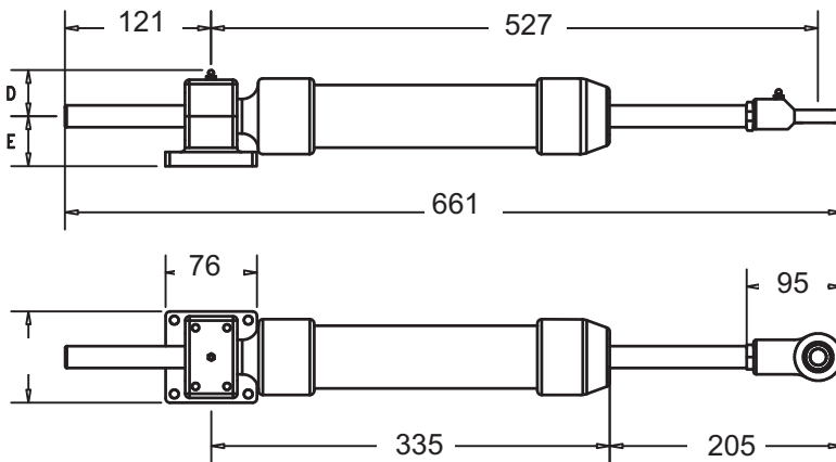
Model 213 Cylinder dimensions
