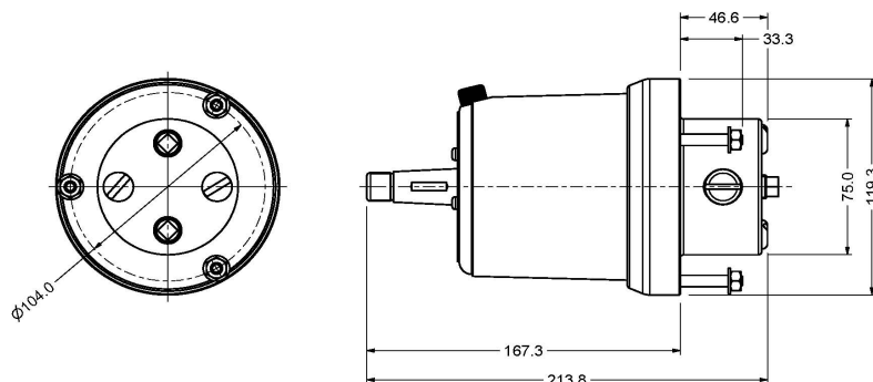
Model 401 and 402 Helm pump dimensions
