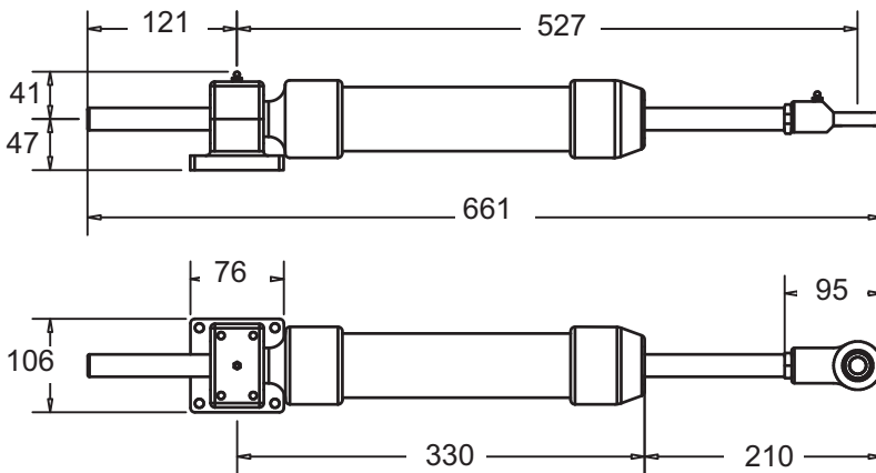
Model 210 Cylinder dimensions
