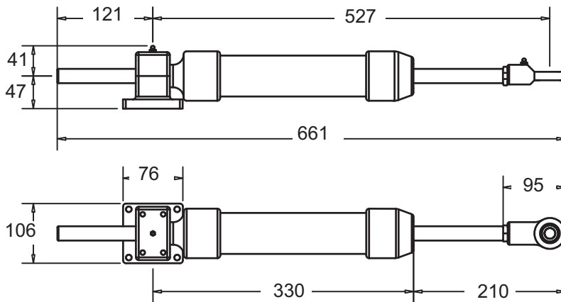
Model 216 Cylinder dimensions
