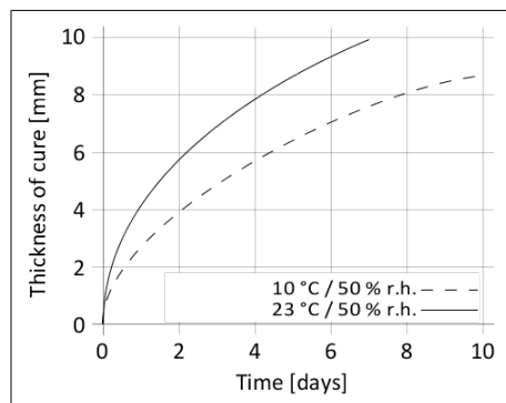
Diagram: Curing speed Sikaflex®-291
